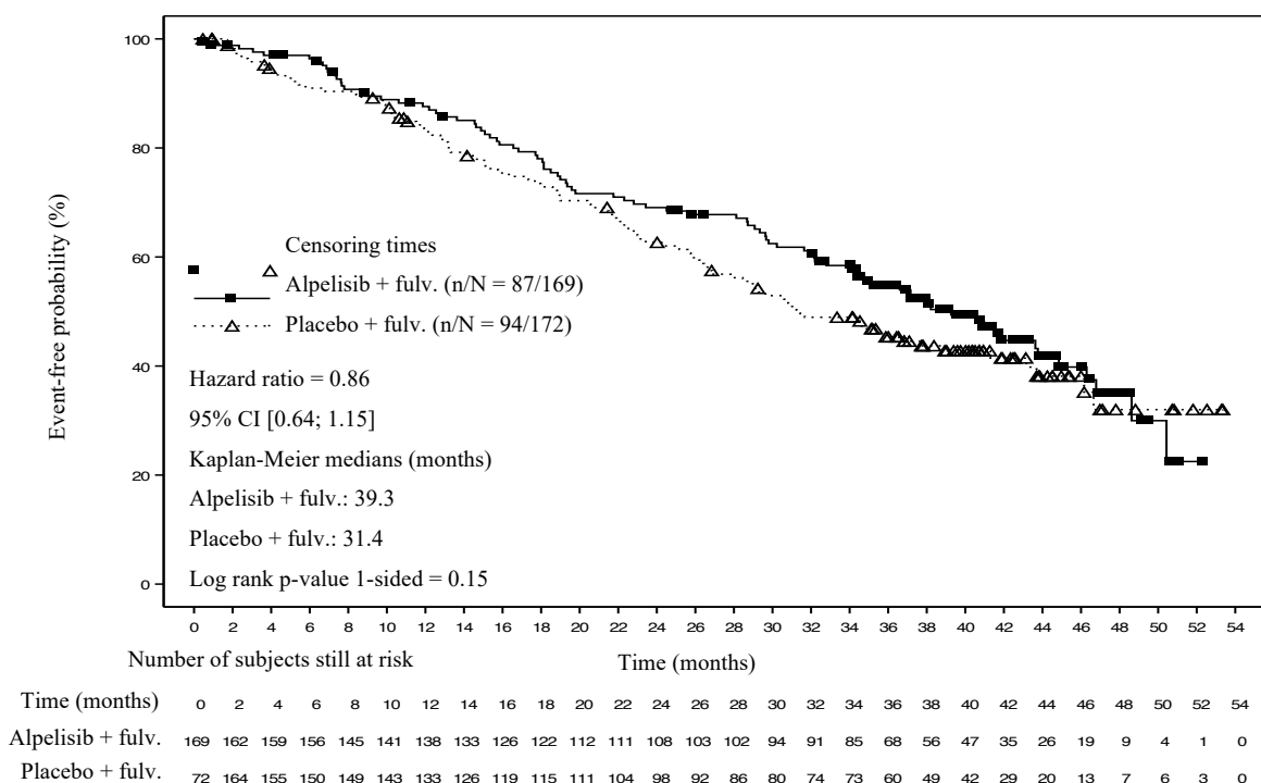
Figure 2 Study C2301 key secondary analysis – Kaplan-Meier plot of OS (FAS, PIK3CA mutant cohort) with cut-off date of 23-Apr-2020
